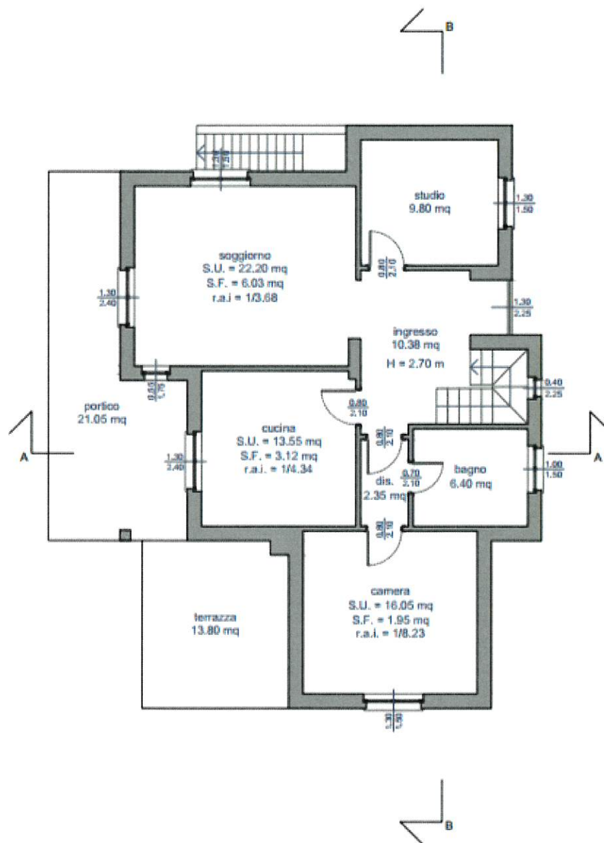
PIANO TERRA
